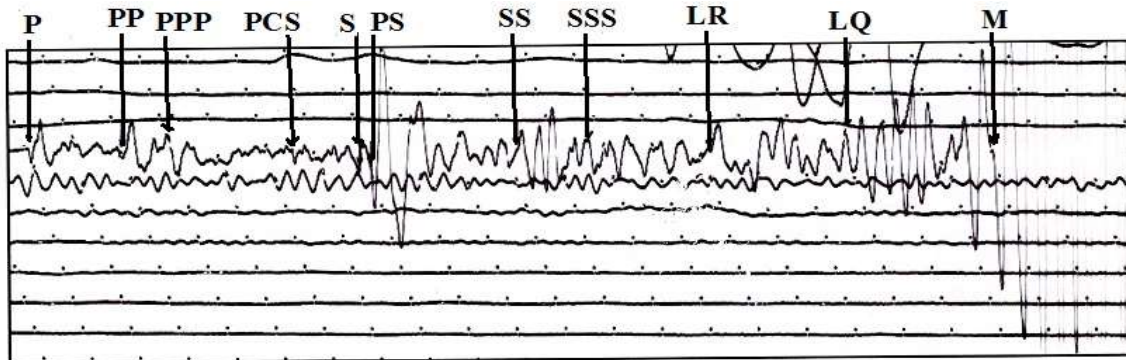
Fig. 4: Different earthquake phases with long epicentral distance
